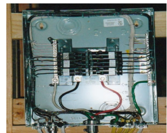
Panel Box
